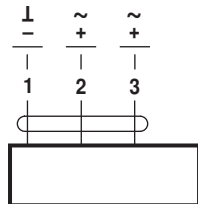
NM24A.. NM72A..
