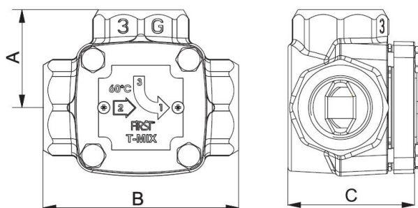
3-way thermic loading valve T-MIX
