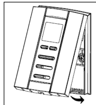
3. Locate lugs and clip the thermostat onto the backplate
