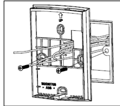
1. Locate the wallplate and pull through the wires
