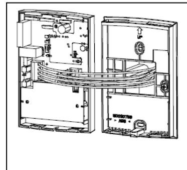
2. Complete the wiring onto the terminal blocks
